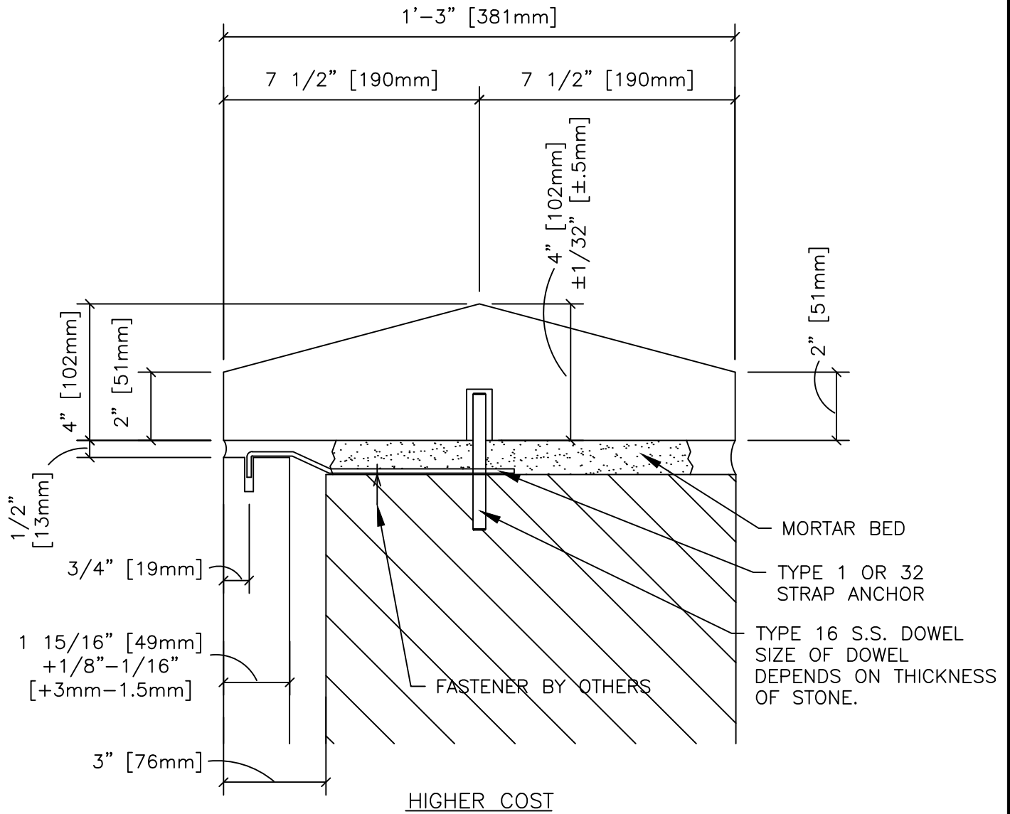
COPING WITH TWO WAY SLOPED TOP
