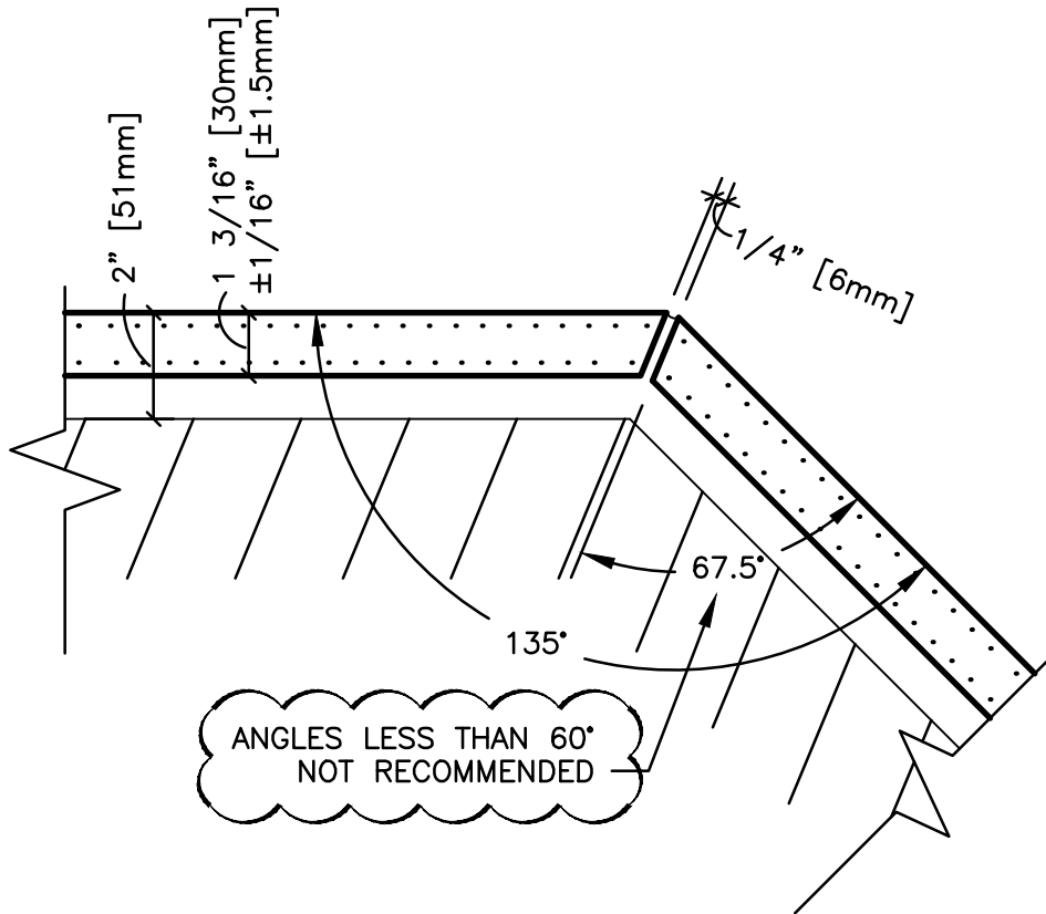
MITER OUTSIDE CORNER
