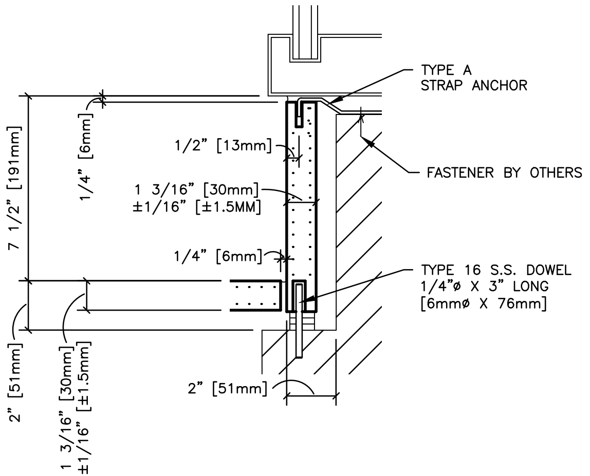
BASE DETAIL – ANCHOR AT TOP AND BOTTOM
