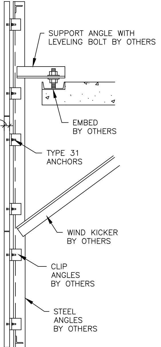
SECTION
